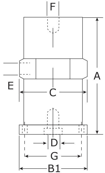
Square Base Dimensions
